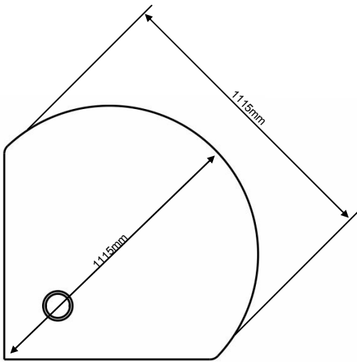
Underside of tray
